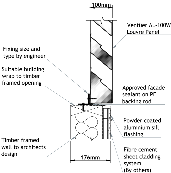
AL-100W (CHANNEL FRAME) SILL DETAIL 03 SCALE 1 : 8
