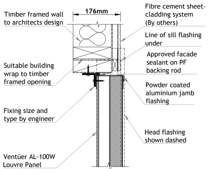
AL-100W (CHANNEL FRAME) JAMB DETAIL 02 SCALE 1 : 8
