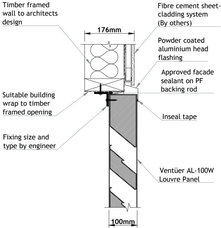
AL-100W (CHANNEL FRAME) HEAD DETAIL 01 SCALE 1 : 8
