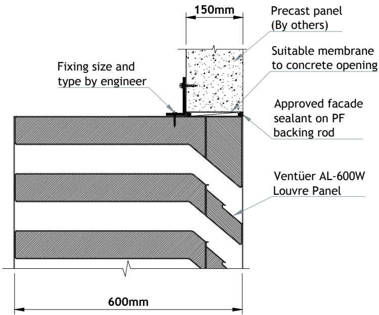
AL-600W (CHANNEL FRAME) HEAD DETAIL 01 SCALE 1 : 10
