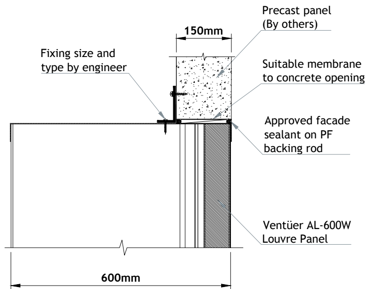
AL-600W (CHANNEL FRAME) JAMB DETAIL 02 SCALE 1 : 10
