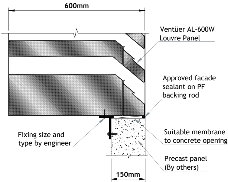
AL-600W (CHANNEL FRAME) SILL DETAIL 03 SCALE 1 : 10
