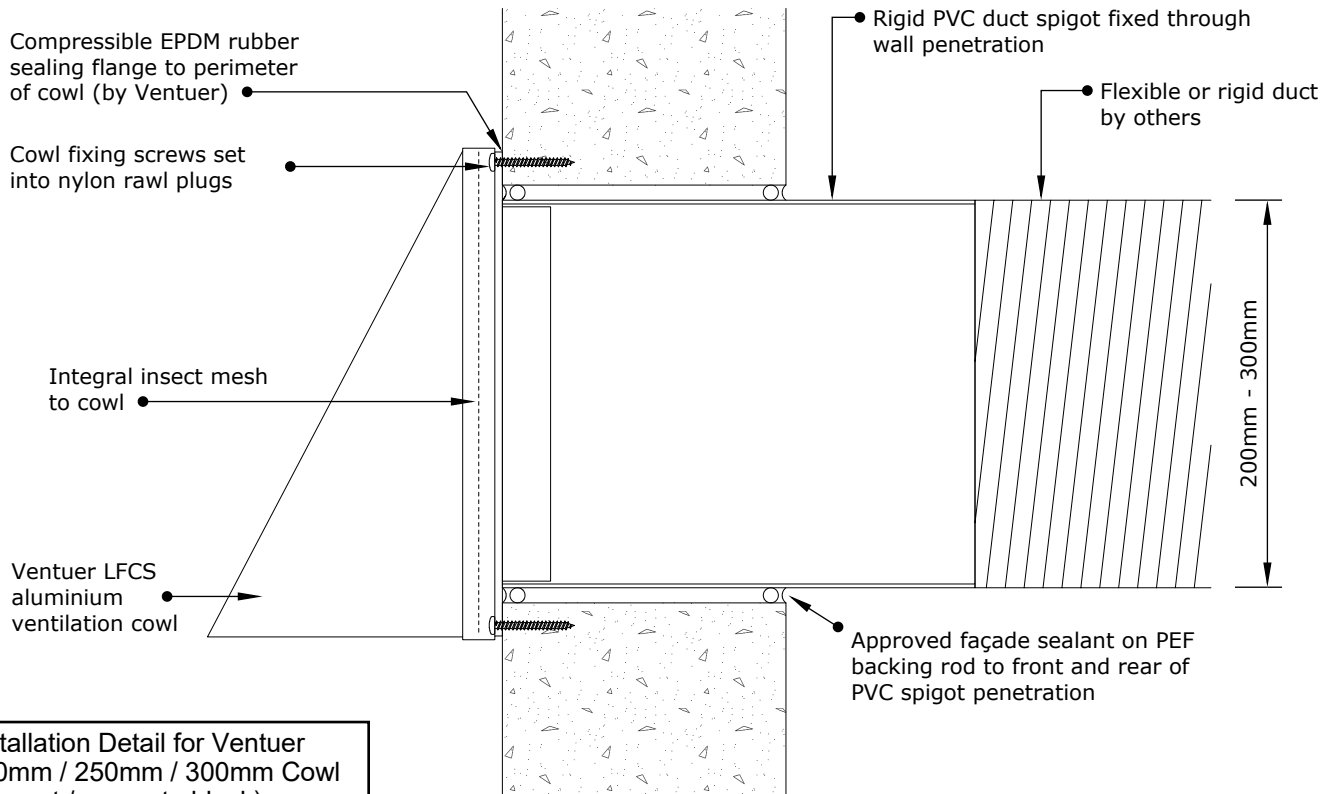
Installation Detail for Ventuer 200mm / 250mm / 300mm Cowl (cladding over drained cavity)
