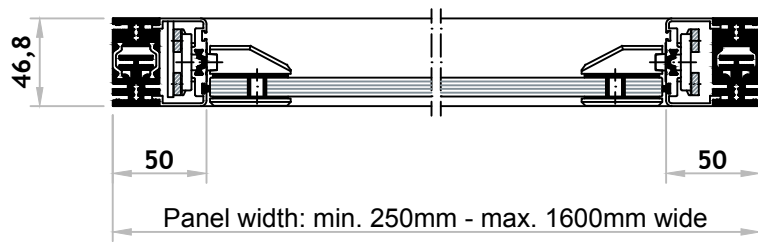
HORIZONTAL SECTION
