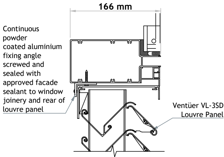
VL-3SD (FLANGED FRAME) HEAD DETAIL 01 SCALE 1 : 4
