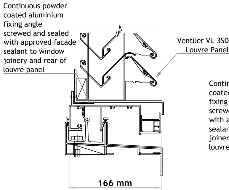
VL-3SD (FLANGED FRAME) SILL DETAIL 03 SCALE 1 : 4
