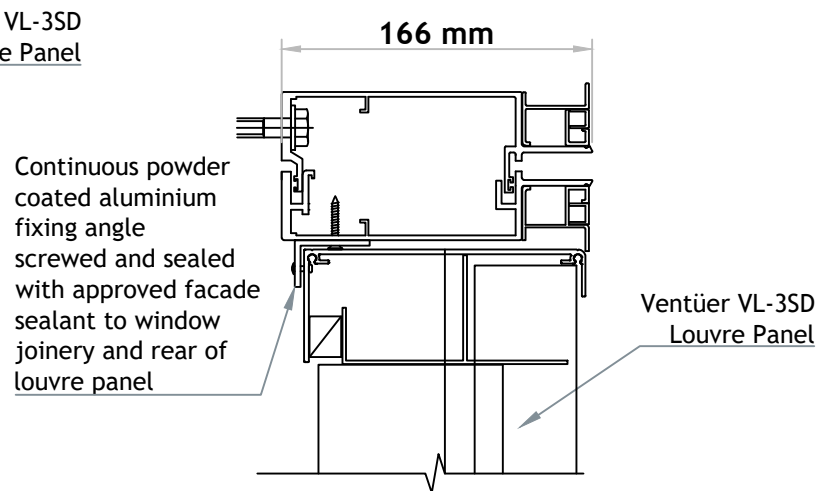
VL-3SD (FLANGED FRAME) JAMB DETAIL 02 SCALE 1 : 4
