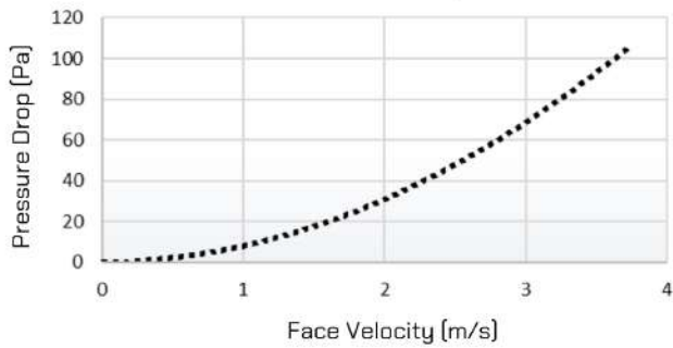
VL-50PL1 Pressure Drop
